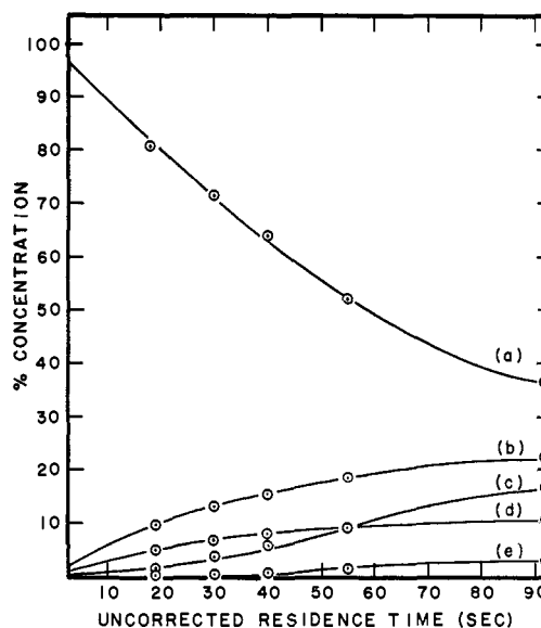
Figure 3. Composition of pyrolysate formed from N - \alpha -methylallylpyrrole at 483.8° vs. time: (a) N - \alpha -methylallylpyrrole, (b) 3- trans -crotylpyrrole, (c) 2- trans -crotylpyrrole, (d) 2- \alpha -methylallylpyrrole, and (e) 3- \alpha -methylallylpyrrole.
