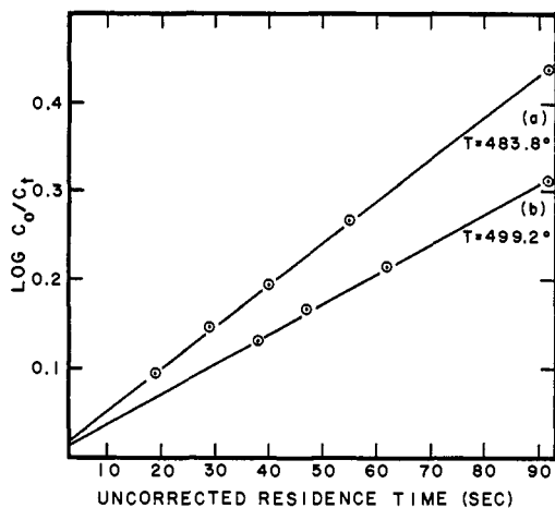
Figure 1. First-order plots for the pyrolysis of N - \alpha -methylallylpyrrole at 483.8° (a) and N - trans -crotylpyrrole at 499.2° (b).
