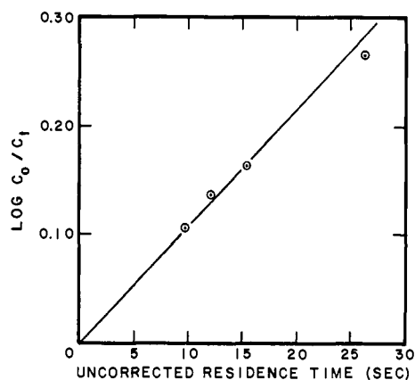
Figure 2. First-order plot for the pyrolysis of 2- \alpha -methylallylpyrrole at 486.6°.
