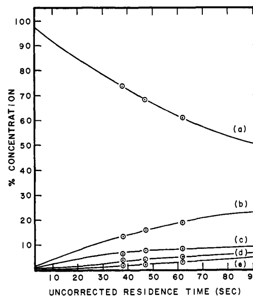
Figure 4. Composition of pyrolysate formed from N - trans -crotylpyrrole at 499.2° vs. time: (a) N - trans -crotylpyrrole, (b) 2- trans -crotylpyrrole, (c) 3- \alpha -methylallylpyrrole, (d) 2- \alpha -methylallylpyrrole, and (e) 3- trans -crotylpyrrole.
